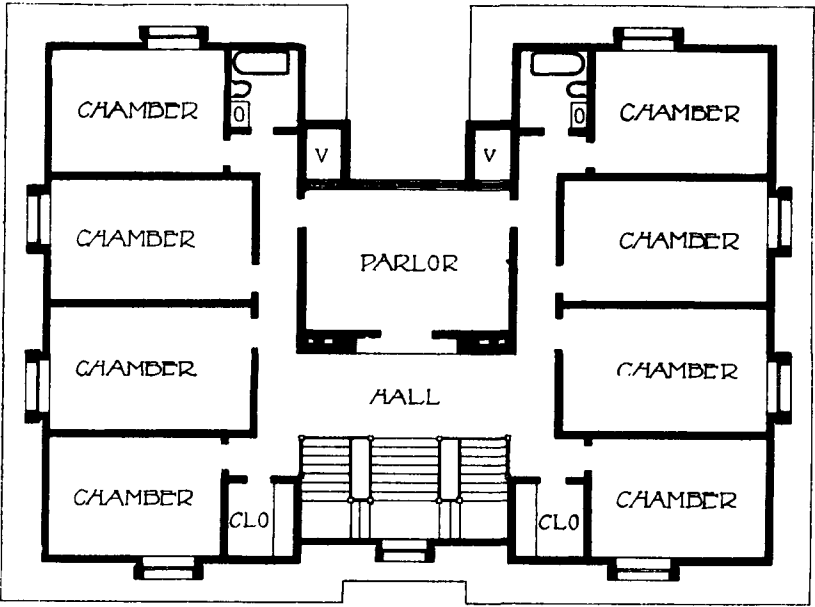
THIRD FLOOR
